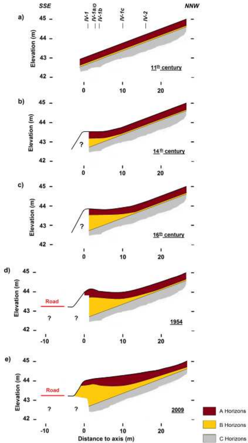
Figure 11. Scenario for lynchet L1 development: L1 morphology in (a) 11 th century, (b) 14 th century, (c) 16 th century, (d) 1954 and (e) 2009. (After Chartin, 2011).
