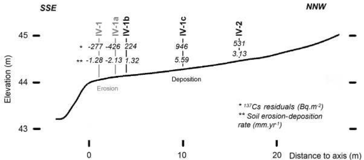
Figure 10. Topographic cross-section along sample transect IV in lynchets L1 and related measured 137 Cs residuals.
